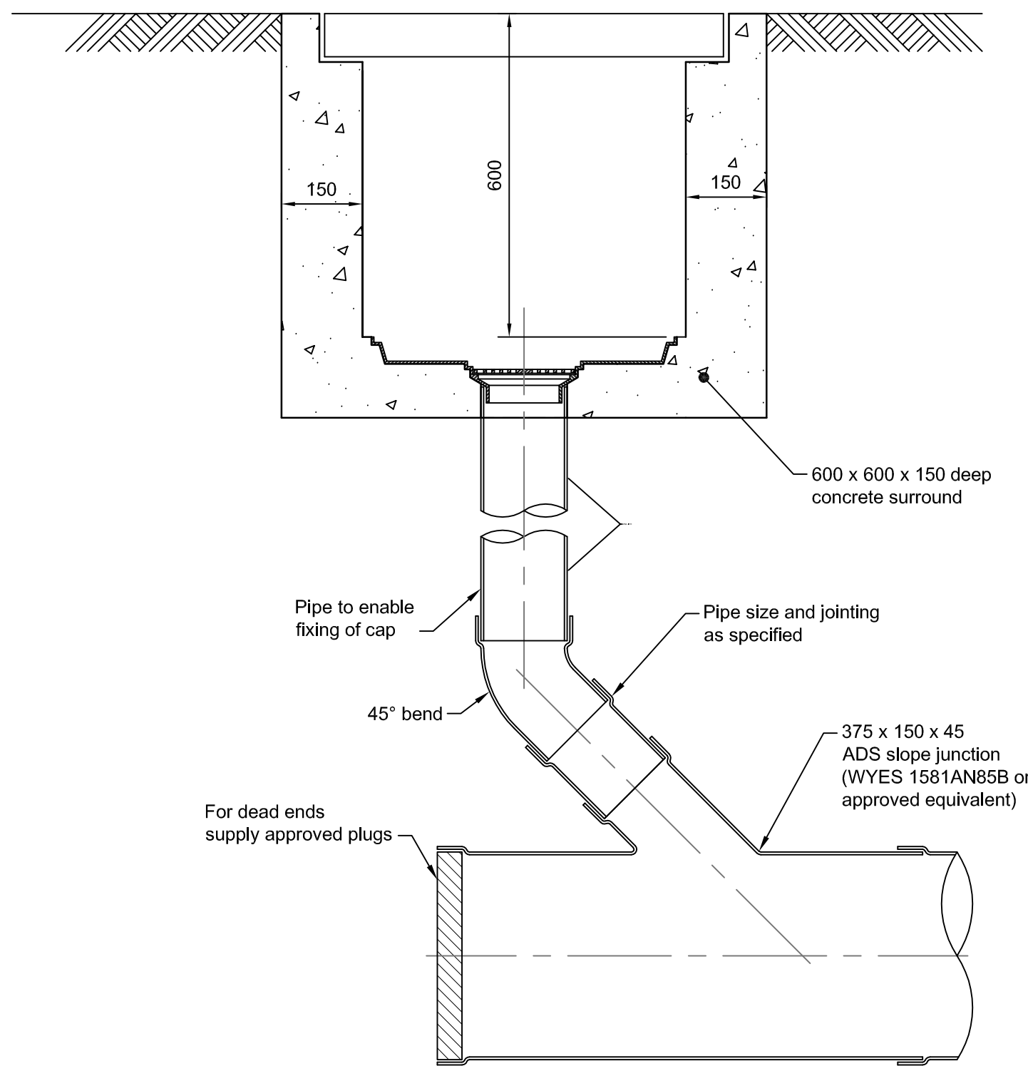
Surface Inlet Connection to Stormwater Drainage Pit Type A
