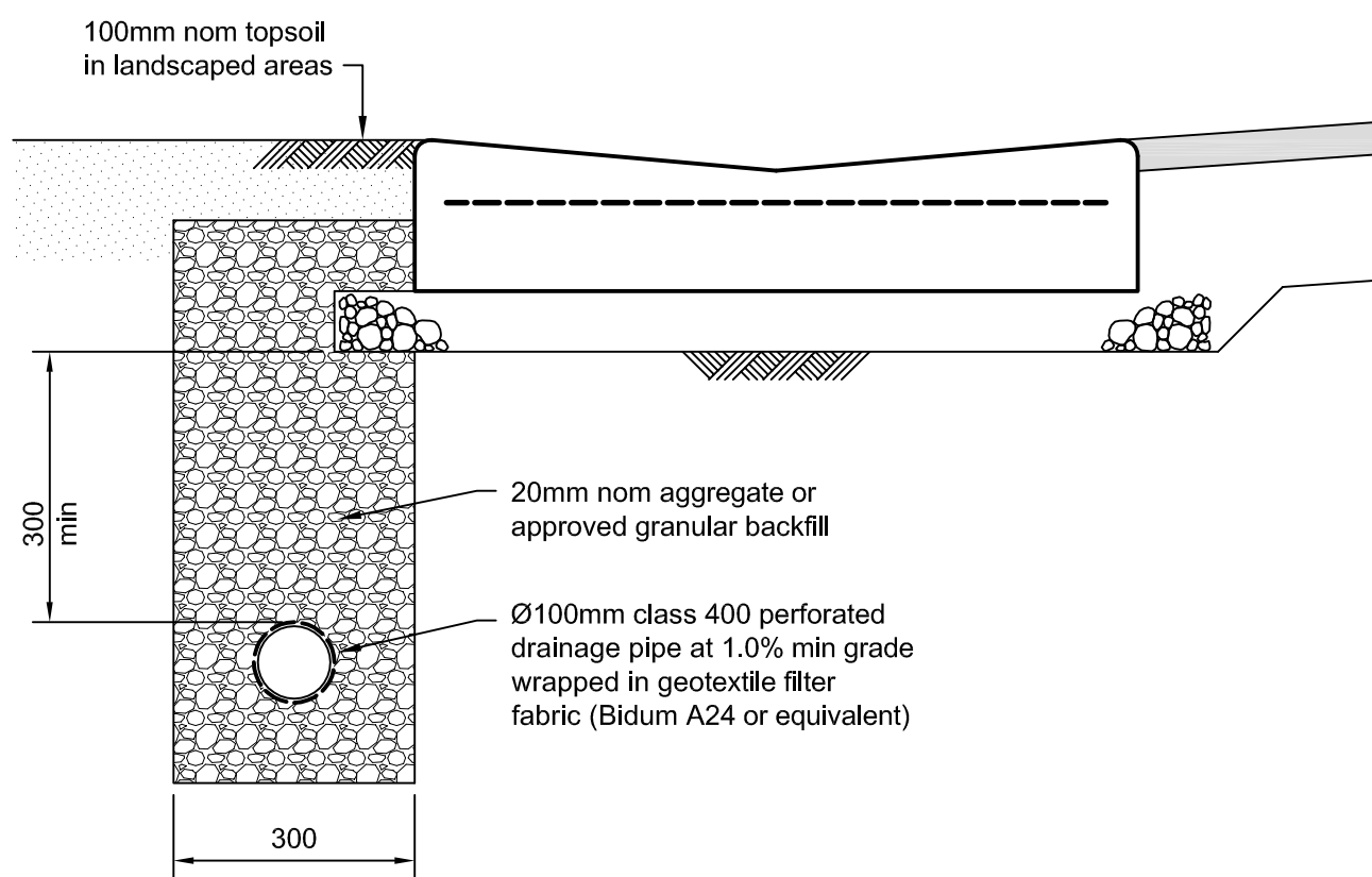
Subsoil Drainage behind Kerbs
