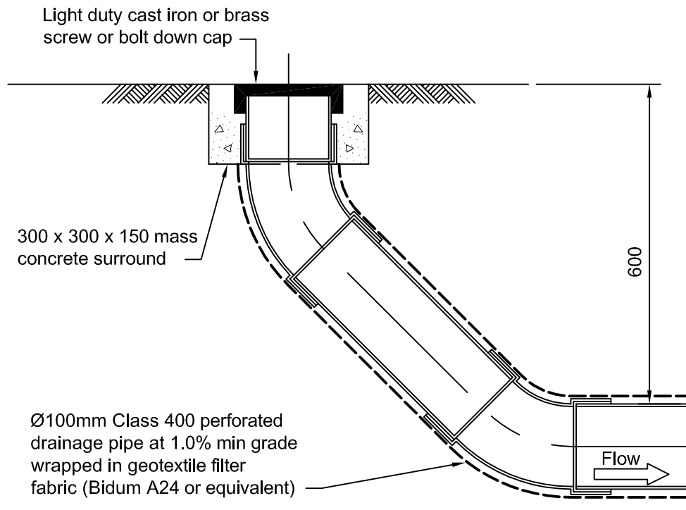
High End Riser (HER)
