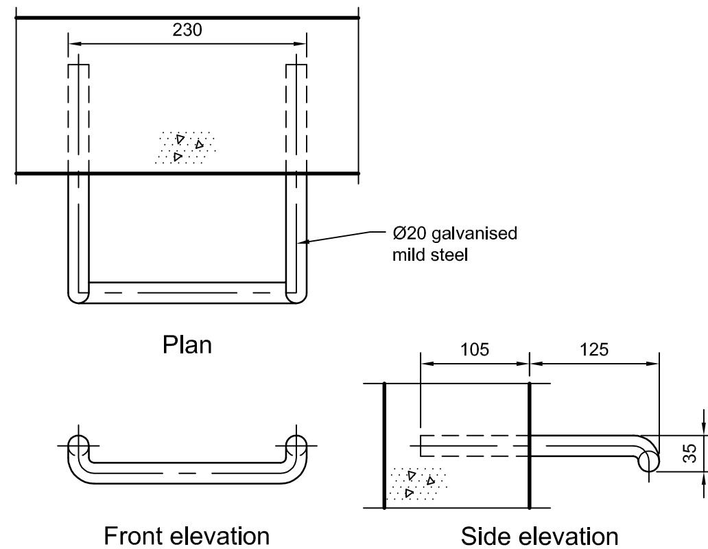
Step iron detail
