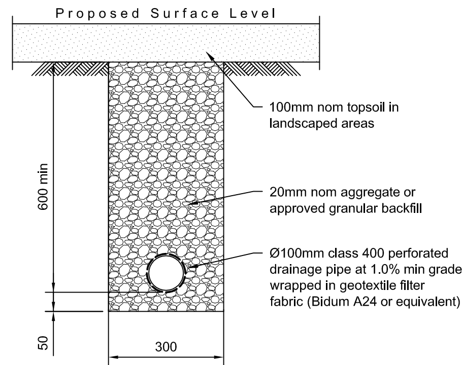
Subsoil drainage in Landscaped Areas
