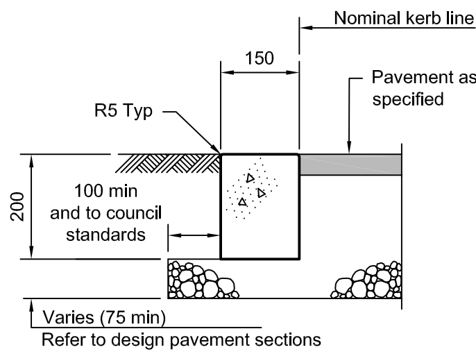
Flush Kerb (FK)
